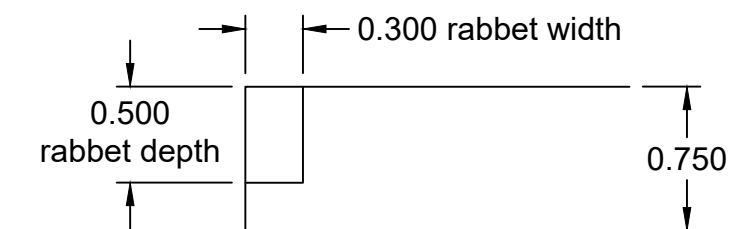
RABBET DETAIL
